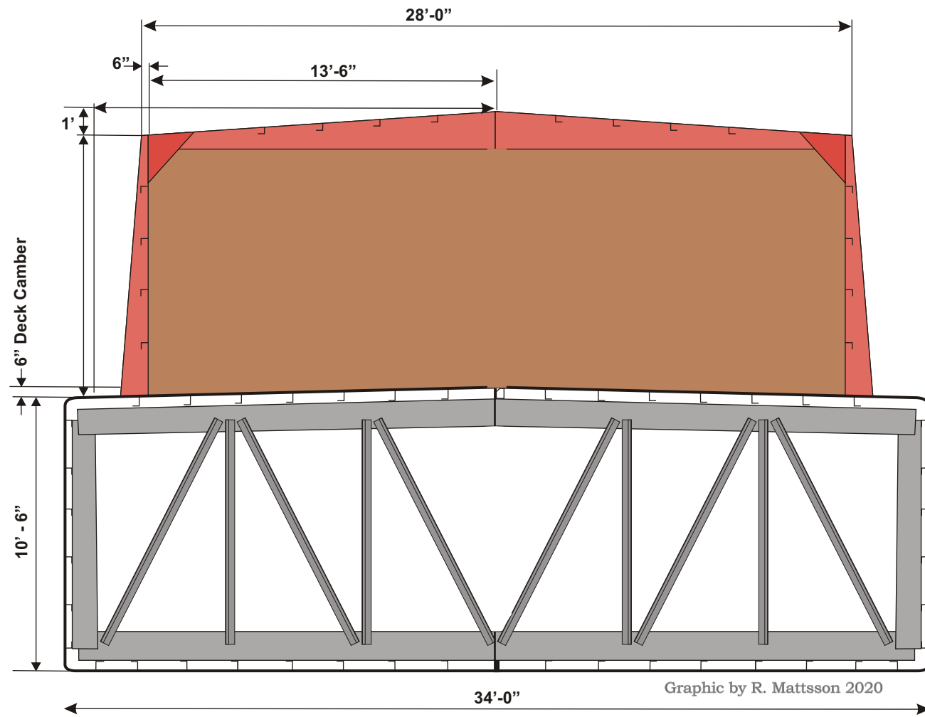
Typical Transverse Section
