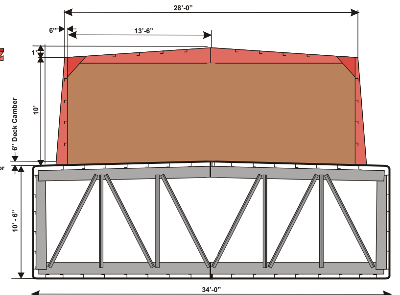
Typical Transverse Section
